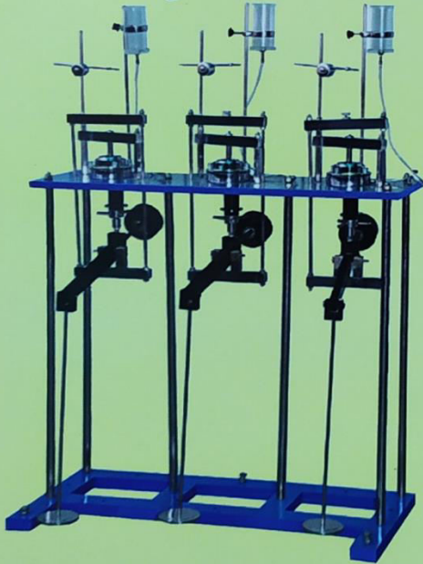
Consolidation Test Apparatus
