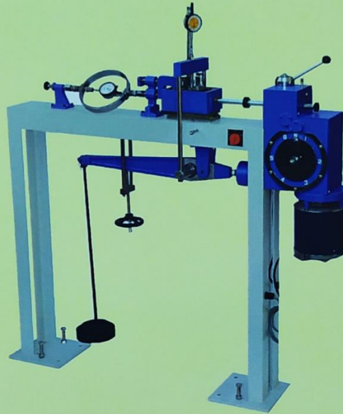
Direct Shear Test Apparatus
