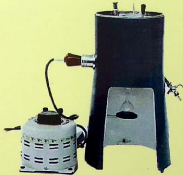
Redwood Viscometer
