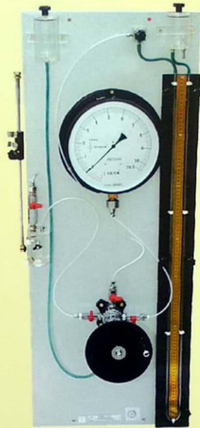
Pore Pressure apparatus
